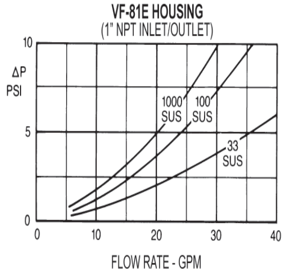
FLOW RATE (USGPM) VS. PRESSURE DROP AT VARIOUS VISCOSITIES FOR EMPTY VF-81E VESSEL (NO CARTRIDGE INSTALLED)
